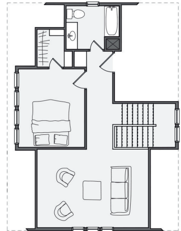
Third Floor
